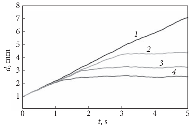
Fig. 4. Results of modeling the effect of ultrasound on the displacement of ore particle 4 relative to particle 3: 1 — displacement of particle \alpha ; 2 — displacement of particle \beta , ultrasound power P_1 = 100 W; 3 — displacement of particle \beta , ultrasound power P_2 = 125 W; 4 — displacement of particle \beta , ultrasound power P_3 = 150 W
