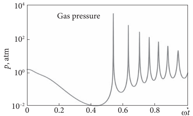
Fig. 1. Pressure change during cavitation collapse of a gas bubble
