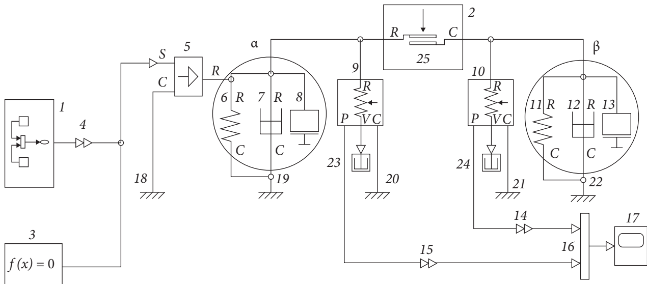
Fig. 3. Scheme of the modeling of the ultrasonic effect on the interaction of crushed ore particles in the pulp
