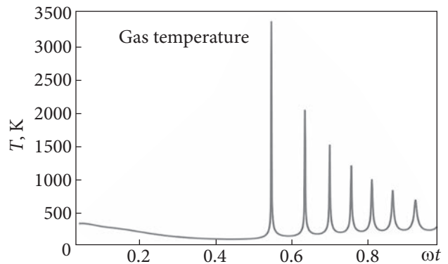
Fig. 2. Temperature change during the cavitation collapse of a gas bubble
