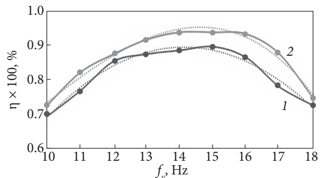
Fig. 5. The results of ultrasonic influence on the process of wet fine screening of ore: 1 — without ultrasonic irradiation; 2 — with ultrasonic irradiation
