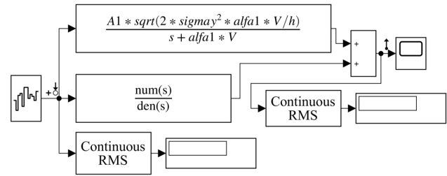
Fig. 1. Subsystem for calculating the values of a road's micro profile by the time function
